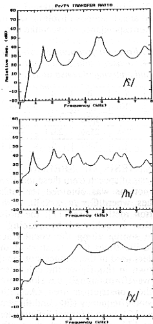
Figure 4. Transfer functions calculated from the idealized area functions. The source for /ʕ/ is both at the glottis and at 1 cm after the constriction (hence two transfer functions). For /ʕ/ and /h/ the source is at the glottis only, and for /χ/ it is placed at 1 cm after the constriction.
